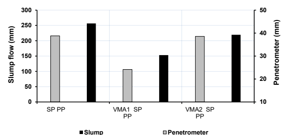
Fig. 11: Effect of VMAs on slump flow and penetration
