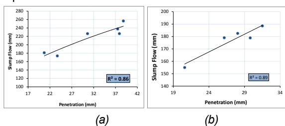
Fig. 13: Relationship between slump flow and penetrometer (a) (different PP and SP), (b) (with and without SF)
