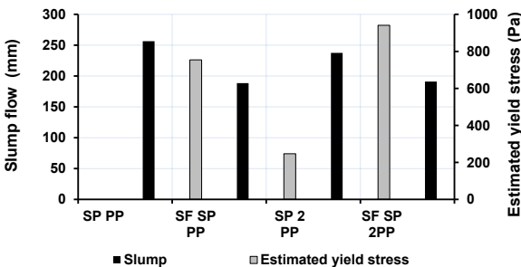
Fig. 7: Effect of SF on slump flow diameter, penetration and estimated yield stress
