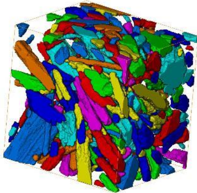
Figure 88 - 3D reconstruction of the sunflower aggregates within the meta-kaolin binder paste
