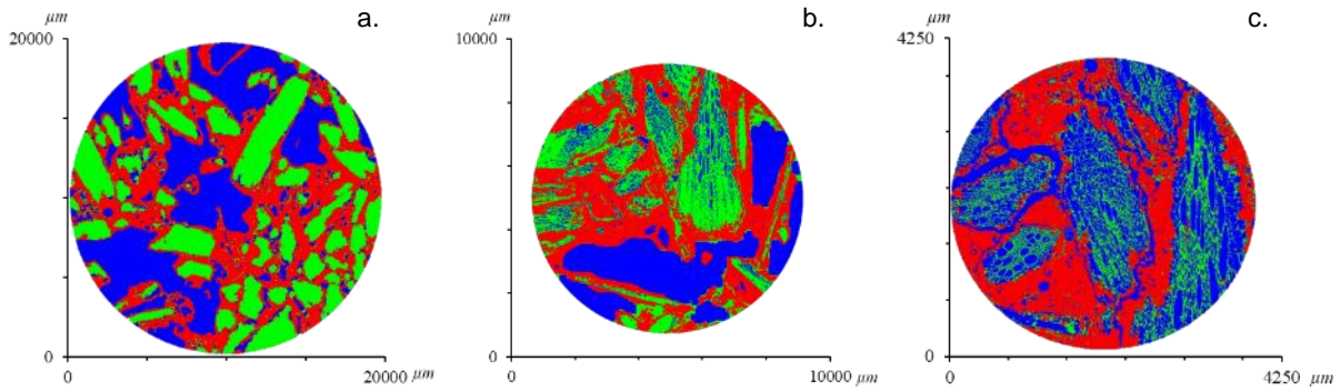
Figure 87 - Identification of binder (red), aggregate (green) and void (blue) phases in MS composite for three different scan resolutions with voxel sizes of (a) 19.9 μm, (b) 10 μm and (c) 4 μm
