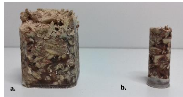
Figure 84 - Sunflower-based samples (a) prismatic sample with a base of 2.33 x 2.33 cm 2 and (b) cylindrical sample with a diameter of 8.8 mm.
