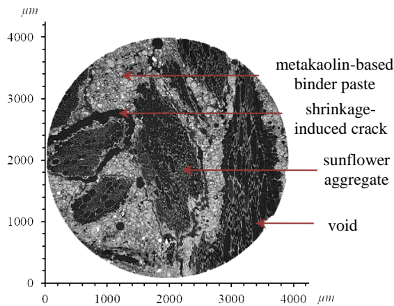
Figure 86 - X-ray tomography slice of MS concrete (voxel size of 4 \mu\text{m} )
