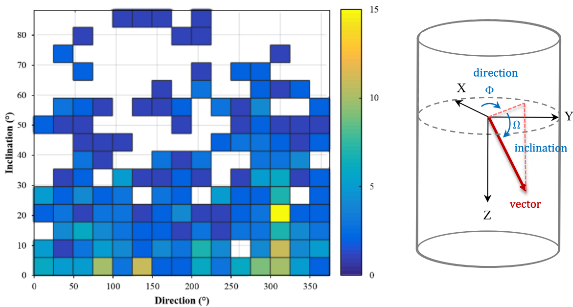
Figure 90 - Spatial orientation of particles: (a) 2d normalized histogram of direction versus inclination and (b) definition of direction and inclination.
